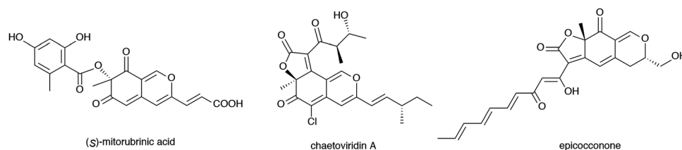
Fig. 1 Azaphilone compounds.
