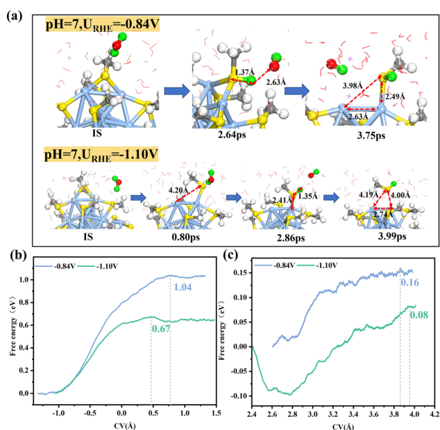
Fig. 1 (a) Schematic of local structures formed during adsorption of *H onto the S site and during Ag–S bond breaking in \text{Ag}_{25}(\text{SR})_{18} at U_{\text{RHE}} = -0.84 \text{ V} and -1.10 \text{ V} . (b) Integral free energy curves for *H adsorption and (c) Ag–S bond breaking at U_{\text{RHE}} = -0.84 \text{ V} and -1.10 \text{ V} , respectively. The Ag, S, C, O and H atoms are shown as pale blue, yellow, grey, red and white spheres, respectively. The H from the attacking \text{H}_2\text{O} is colored in green.
