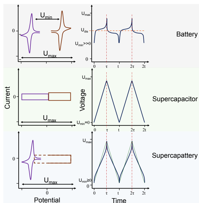
Figure 3. Illustration of CVs of electrodes and GCD profiles of two-electrode cells of battery, supercapacitor and supercapattery. (Redrawn from Ref. 50 )
