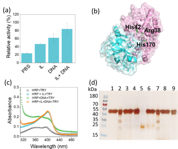
Fig. 3 (a) Relative activity of HRP after incubation with 6 μM TRY at 37 °C for 24 h in the presence of various solvent systems. (b) Docking results of TRY binding to HRP. HRP is shown in magenta and catalytic residues highlighted as green sticks. TRY is shown in cyan. (c) UV-Vis spectra of HRP after incubation with TRY. (d) SDS-PAGE analysis of HRP with and without TRY digestion in various solvent systems. Lane 1: IL + HRP; lane 2: DNA + HRP; lane 3: IL + DNA + HRP; lane 4: HRP in PBS; lane 5: TRY in PBS; lane 6: IL + HRP + TRY; lane 7: DNA + HRP + TRY; lane 8: IL + DNA + HRP + TRY; lane 9: HRP + TRY.
