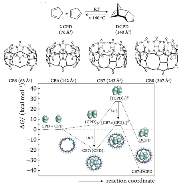
Fig. 1 Cucurbit[n]urils with varying cavity sizes used for catalyzing the Diels–Alder reaction. Adapted from ref. 31 with permission from ACS Publishing Group.
