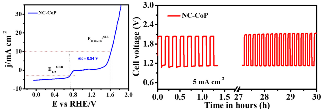
Fig. 8 (a) Polarization curves illustrating the bifunctional electrocatalytic activity of NC-CoP. (b) Charge–discharge cycling performance at 5 \text{ mA cm}^{-2} of the rechargeable ZAB.
