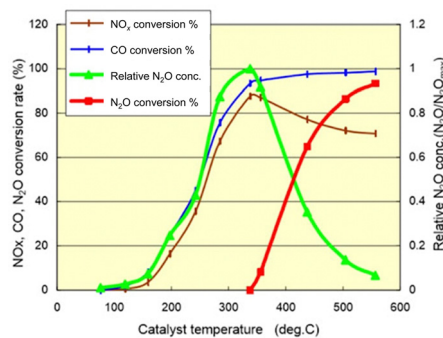
Fig. 3 Conversion of exhaust pollutant species over a TWC. Cited from National Traffic Safety and Environment Laboratory. Research on low emission vehicles: effect of catalyst temperature behaviour on nitrous oxide (N 2 O) emissions in cold climates.
