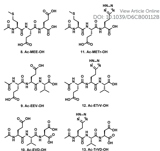
Fig. 5. ‘3-mer’ peptides 8–13 derived from parent peptides 1 and 2 .
