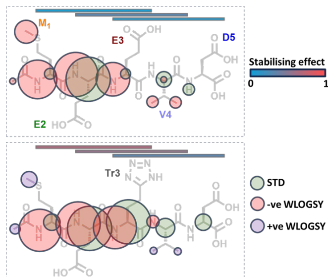
Fig. 11. Summary of the SLiM observed 'fingerprinting' of the Hop TPR2A -1 (top) and Hop TPR2A -2 (bottom) complexes, respectively. The coloured bars represent the stabilising effect of each overlapping 3-mer, relative to the data obtained for apo Hop TPR2A (0) and the Hop TPR2A -2 complex (1). Calculations in Table S1. Bubble colour represents the mechanism of NOE magnetization, while bubble diameter is proportional to signal intensity. STD signals below the experimental mean and WLOGSY signals, which were suppressed to 0% but not inverted were excluded.
