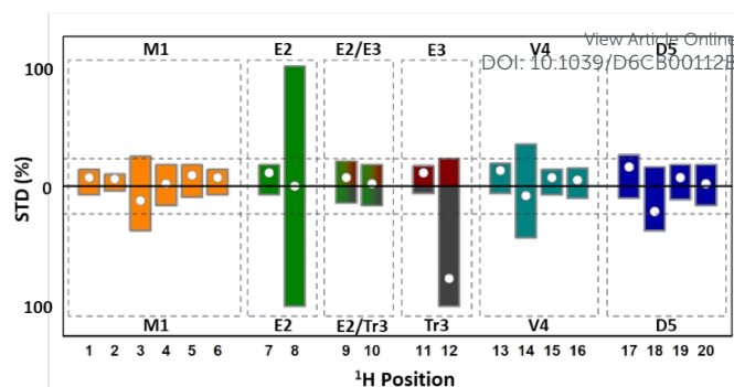
Fig. 9. Comparative analysis of STD NMR data of the Hop TPR2A -1 (phased up) and Hop TPR2A -2 (phased down) complexes, respectively. Each residue is boxed off and shown in a distinct colour for clarity. The ambiguously assigned H-9 and H-10 protons are grouped together. ^1\text{H} position correlates to numbering in Fig. 1B. The horizontal dashed line depicts the mean STD intensity for each experiment. The height of each bar corresponds to the relative magnitude of the STD signal, whereas the white circles indicate the difference in magnitude for corresponding signals between the Hop TPR2A -1 and Hop TPR2A -2 experiments. In both complexes, the E2 \alpha -proton (H-8) was the most prominent signal, indicating a central role in binding for both peptides. The most noticeable change was observed between the H-12 protons of each peptide, suggesting that the Tr3 \alpha -proton makes a significant new interaction with Hop TPR2A . In addition, the changes observed between H-17 and H-18 for peptides 1 and 2, suggest a change in conformation in this region.
