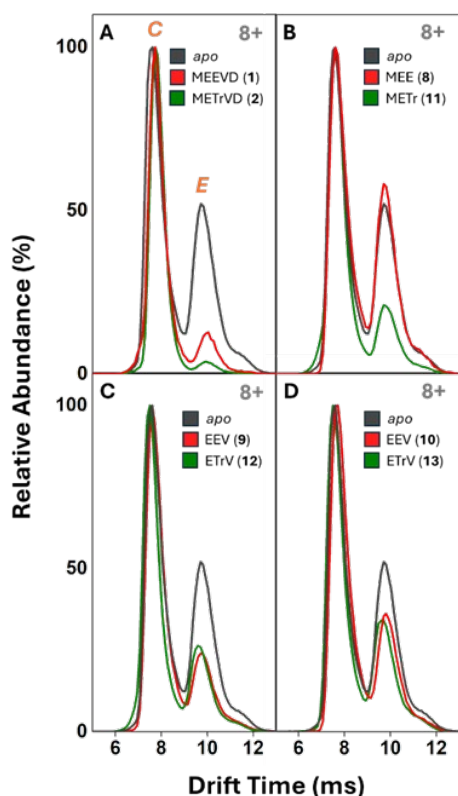
Fig. 4A. Arrival time distributions of the 8 + charge state of the native mass spectra of apo Hop TPR2A and the complexes with peptides 1 and 2 showing the presence of a compact (C) and extended (E) conformer of Hop TPR2A . These data indicate that complexation with peptides 1 and 2 promotes the gas-phase stability of the C conformer. B – D. Arrival time distributions of the 8 + charge state of the native mass spectra of peptide ‘3-mers’ 8–13 in complex with Hop TPR2A overlaid with the data for apo Hop TPR2A . Most notably, peptide 8 (MEE) was unable to influence gas phase stability of the C conformer.
