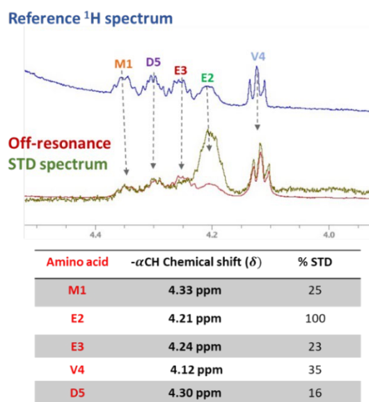
Fig. 8. Stacked 1D ^1\text{H} expansions of Hop TPR2A -1 complex. The reference ^1\text{H} spectrum is shown in blue, while the off-resonance and STD spectra are shown in red and green, respectively. The STD amplification factor for each unique signal was calculated as the percentage of signal in the off-resonance spectra over the signal intensity in the STD spectrum.
