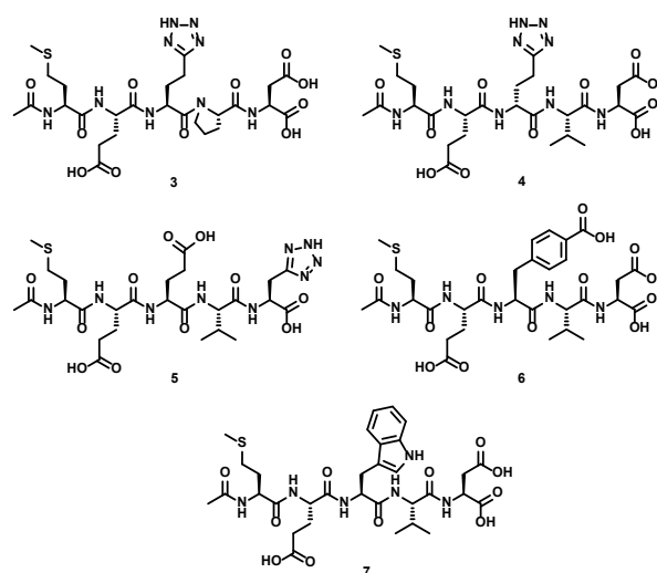
Fig. 2. Selected peptides from a previously reported SAR study which indicated that apart from some interaction plasticity at residue 3, (e.g. peptides 6 and 7 ) very little alteration from the core motif is tolerated. 23
