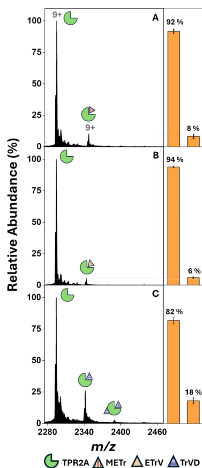
Fig. 7. nMS of the 9 + charge state of a 1:5 mixture of Hop TPR2A and peptides 11 (A), 12 (B) and 13 (C) in 50 mM NH 4 OAc solution. Accompanying these spectra are complexation ratios calculated by combining the magnitude of bound and unbound protein across both the 8 + and 9 + charge state. These data are an average of three independent replicates. Error bars represent the standard deviation of these replicates. The same negative influence on binding is observed as in Fig. 6.
