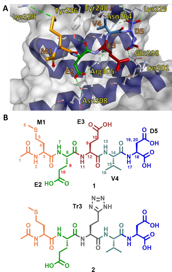
Fig. 1A: X-ray co-crystal structure of Ac-MEEVD-OH ( 1 ) bound to Hop TPR2A (PDB 1ELR). This interaction is dominated by a series of salt bridges formed between basic residues found in the binding groove of Hop TPR2A and the acidic residues of 1 including the 'carboxylate clamp' formed by the terminal D5 residue. B: Peptide 1 is an acetylated analogue of the naturally occurring MEEVD SLIM and has no PPI inhibitory activity. Peptide 2 is a PPI inhibitory non-natural analogue of 1 . Peptides are coloured per residue to match data shown in Figs. 8, 9 and 10. Numbering of structures correlates to numbering used for NMR structural elucidation.
