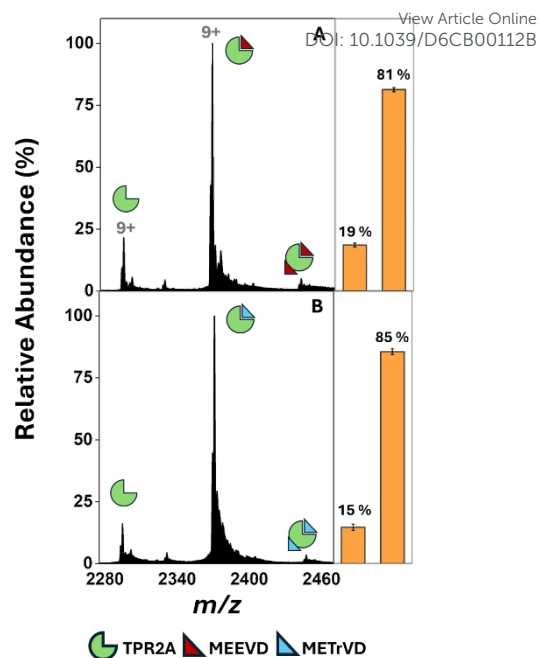
Fig. 3. nMS of the 9 + charge state of a 1:5 mixture of Hop TPR2A and peptides 1 (A), and 2 (B) in 50 mM NH 4 OAc solution. Accompanying these spectra are complexation ratios calculated by combining the magnitude of bound and unbound protein across both the 8 + and 9 + charge state. These data are an average of three independent replicates. Error bars represent the standard deviation of these replicates. Despite neither peptide fully saturating Hop TPR2A evidence of a second binding event emerged at this relative concentration.
