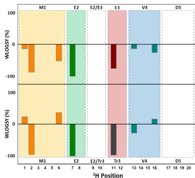
Fig. 10. Comparative analysis of WLOGSY NMR data of the Hop TPR2A -1 (top) and Hop TPR2A -2 (bottom) complexes respectively. Figure formatting matches Fig. 9. Regions where WLOGSY signals were detected are highlighted in colour. In both complexes, the E2 NH proton (H-7) was the most prominent signal, again like the STD data indicating a central role for E2 in binding for both peptides. The changes in WLOGSY signals, particularly the presence of +ve signals for H-1, H-6 and H-16, indicate substantial changes in the interaction of M1 and V4 with binding site waters for peptide 2 when compared to peptide 1.
