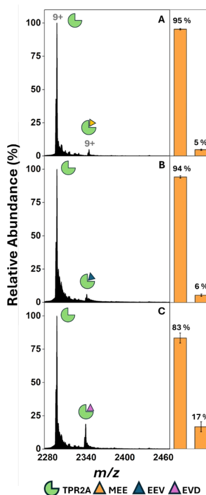
Fig. 6. nMS of the 9 + charge state of a 1:5 mixture of Hop TPR2A and peptides 8 (A), 9 (B) and 10 (C) in 50 mM NH 4 OAc solution. Accompanying these spectra are complexation ratios calculated by combining the magnitude of bound and unbound protein across both the 8 + and 9 + charge state. These data are an average of three independent replicates. Error bars represent the standard deviation of these replicates. These data suggest that the loss of two amino acids from the parent sequence has a disproportionately negative impact on binding.
