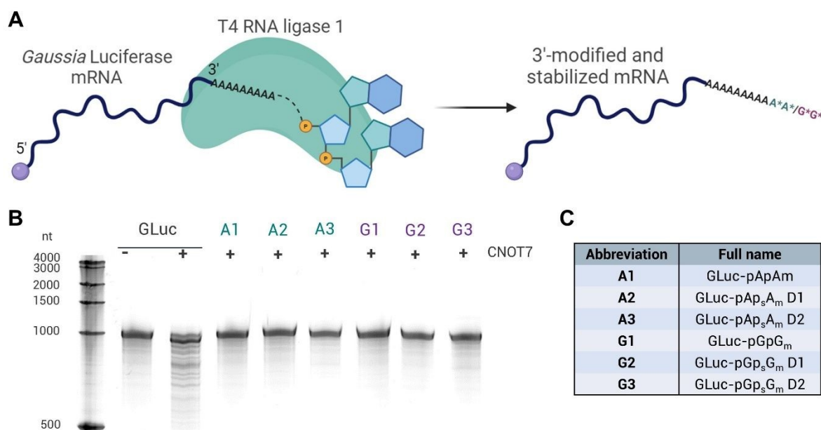
Figure 3. Modification and evaluation of Gaussia Luciferase mRNA. (A) 3' end of Gluc mRNA is modified with different dinucleotides via ligation. (B) PAGE analysis of modified mRNAs, along with unmodified control GLuc mRNA, after 30 minutes of incubation with CNOT7. All modified mRNAs remained stable and full-length after incubation with CNOT7, whereas unmodified GLuc was shortened through removal of its poly(A) tail. Samples were
