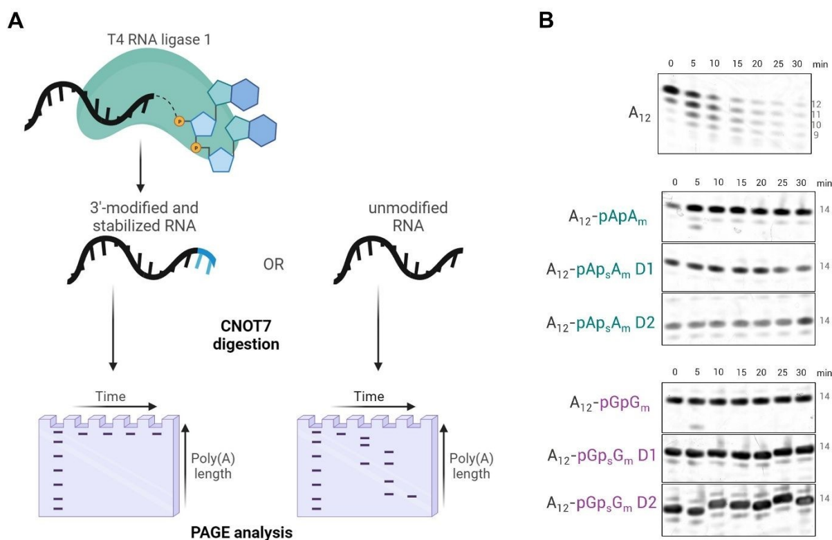
Figure 2. Modification of 3'-end of short RNA with chemically modified dinucleotides. (A) Schematic representation of 3'-end modification of oligonucleotides via enzymatic ligation followed by stability experiments and PAGE analysis. (B) PAGE analysis of ligation products after degradation experiments with CNOT7 deadenylyase. Samples were separated on 18% polyacrylamide urea gel. Gels were stained with SYBR Gold before scanning.
