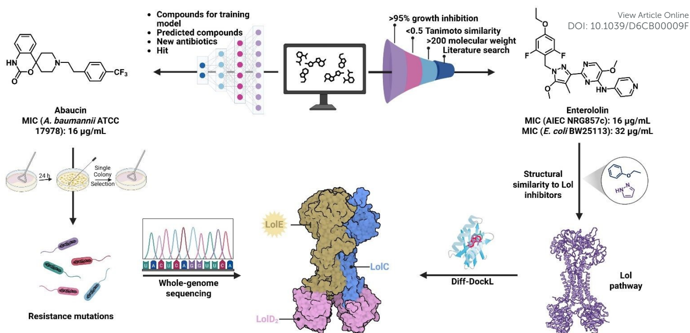
Fig. 4 Overview of the discovery of abaucin and enterololin and identification of their target. Created in BioRender. Lab, W. (2026) https://BioRender.com/f9gw8fl
