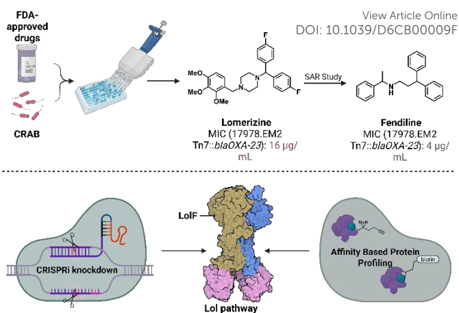
Fig. 6 Overview of the Drug Repurposing screen performed against A. baumannii and the identification of the Lol pathway through CRISPRi knockdown and AbPP. Created in BioRender. Lab, W. (2026) https://BioRender.com/f9gw8fl
