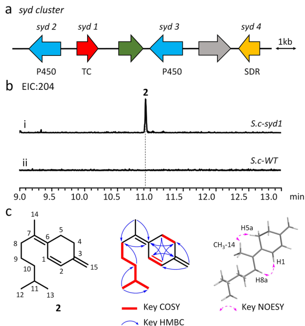
Fig. 2 Functional confirmation of sydl . (a) Organization and proposed function of the syd gene cluster (green: transcription factor, grey: MFS-type transporter). (b) GC-MS analysis showing sydl having catalyzed the formation of 2 . (c) Structure determination of 2 .
