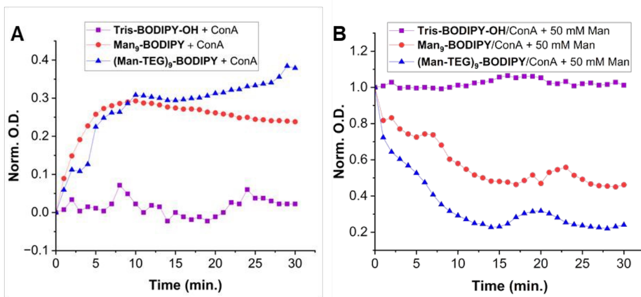
Figure 3. Turbidimetry analysis. A: absorbance ( \lambda = 490 nm) changes over time of a solution ( 20\mu\text{M} ) of Tris-BODIPY-OH (purple line), Man 9 -BODIPY (red line), and (Man-TEG) 9 -BODIPY (blue line) treated with a solution of ConA ( 20\mu\text{M} in HEPES 25 mM, pH 7.6 , 1 mM \text{CaCl}_2 , 1 mM \text{MnCl}_2 ); B: deagglutination over time of glycoBODIPYs/ConA by treatment with a solution of \alpha -O-methyl-D-mannopyranoside ( 50 mM).
