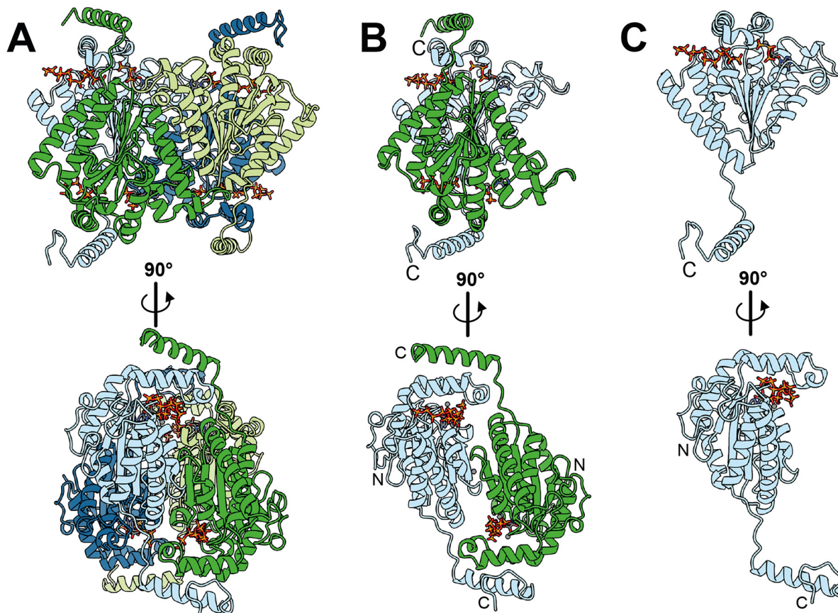
Fig. 3 Overall crystal structure of EbPPK2 (PDB: 9IGQ) at 1.7 Å resolution. (A) EbPPK2 forms a homotetramer (dark and light blue, dark and light green). In each of the active sites, adenosine-5'-[[(β,γ)-methylene]triphosphate (ACP) and polyP are bound. (B) The dimer illustrates that a C-terminal α-helix (clamp) connects two monomers. N-terminus and C-terminus are marked with N and C respectively. (C) Each monomer shows the typical V-shape α-β-fold and one active site with a nucleotide-binding cleft and a polyP-binding tunnel in which two Mg 2+ are bound.
