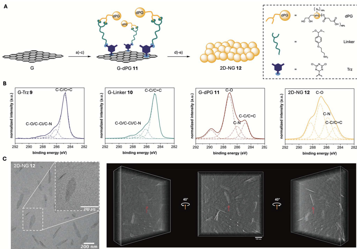
Fig. 2 (A) Schematic illustration and synthetic route for 2D-NG 12. (a) cyanuric chloride, \text{NaN}_3 , NMP, 0 °C to 80 °C, 48 h; (b) DMPA, TEA, DMF, r.t., 48 h; (c) dPG- (\text{N}_3)_{10\%} - (\text{COOH})_{40\%} , PTSA, DMF, r.t., 24 h; (d) tripropargylamine, NaAsc, \text{CuSO}_4 \cdot 5\text{H}_2\text{O} , DMF/ \text{H}_2\text{O} , 50 °C, 24 h; (e) 1 M HCl, r.t., 24 h. (B) Highly resolved C1s XP spectra of G-Trz 9, G-Linker 10, G-dPG 11, 2D-NG 12. The main components are denoted on each spectrum. For further details of the assigned components see Table S3.† (C) TEM image and TOMO of 2D-NG 12 in Milli-Q water at a concentration of 4 \text{mg mL}^{-1} .
