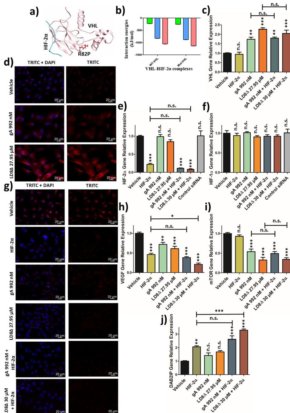
Fig. 6 (a) Crystal structure of the VHL-HIF-2α complex (PDB ID: 6BV8). The Arg82Pro mutation site in VHL protein specific to the SK-RC-45 renal cell carcinoma (RCC) cell line is represented in a red ball and stick model. VHL and HIF-2α proteins are shown in ribbon representation in pink and cyan, respectively. (b) Bar graph showing the average interaction energy of wild-type VHL and mutant VHL with HIF-2α. The total interaction energy (pink) is the sum of van der Waals energy (green) and electrostatic energy (blue). Real-time PCR data showing relative gene expression of (c) VHL (von Hippel-Lindau, responsible for degradation of HIF-α protein), (e) HIF-2α, (f) HIF-1α, (h) VEGF, (i) mTOR and (j) DAB2IP gene in SK-RC-45 cells after treatment with gA, LD8Δ peptide and HIF-2α gene silencing, both in monotherapy and combination therapy at 72 h time point. Immunofluorescence of (d) VHL protein and (g) HIF-2α protein after treatment with gA (992 nM) and LD8Δ peptide (27.95 μM) at 72 h time point compared with untreated SK-RC-45 cells, considered as vehicles. Scale bar = 20 μM. VHL is upregulated at both the gene and protein levels in the presence of both gA and LD8Δ peptide. Both gA and LD8Δ peptide have no influence in downregulating HIF-2α at gene expression level. Both monotherapy and combination therapy did not have any effect in HIF-1α gene expression. Both monotherapy and combination therapy has drastically reduced HIF-2α protein expression. Combination therapy of LD8Δ peptide and HIF-2α gene silencing exhibited significant reduction in VEGF gene expression compared with monotherapy. Both gA and LD8Δ peptide induced significant reduction in mTOR gene expression. Combination therapy of LD8Δ peptide and HIF-2α gene silencing exhibited significant upregulation in DAB2IP gene expression compared with monotherapy. p values are based on one-way ANOVA with Bonferroni post-test (*, p < 0.05; **, p < 0.01; ***, p < 0.001; n.s., not significant compared with vehicle). Results are presented as mean ± SEM.
