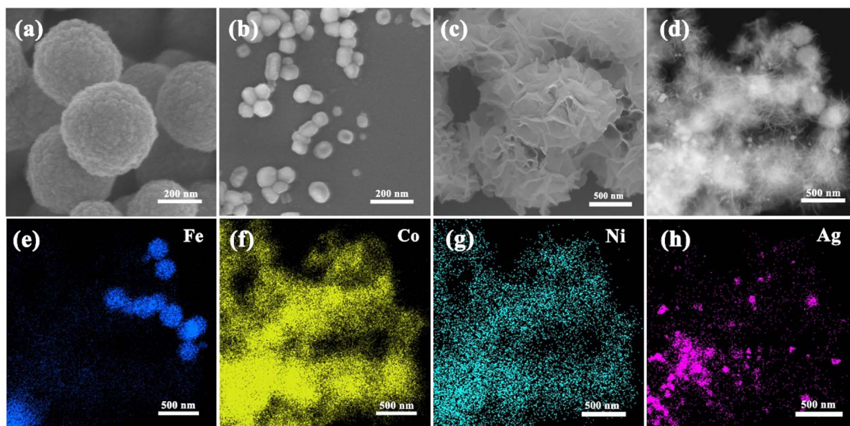
Fig. 1 SEM images of (a) Fe 3 O 4 , (b) Ag NPs and (c) Fe 3 O 4 @CoNi LDH; (d) TEM images of Fe 3 O 4 @CoNi LDH@Ag NPs; and (e–h) EDS elemental mapping spectra of Fe, Co, Ni, and Ag of Fe 3 O 4 @CoNi LDH@Ag NPs, respectively.
