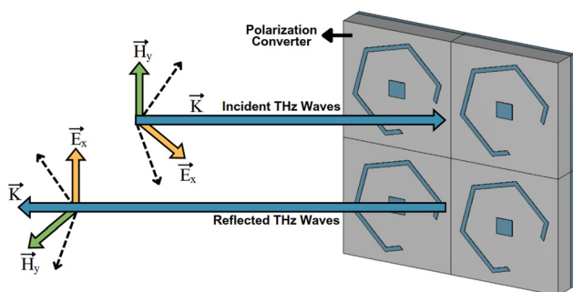
Fig. 2 Illustration of polarization conversion mechanism from incident x polarized to reflected y polarized wave.
