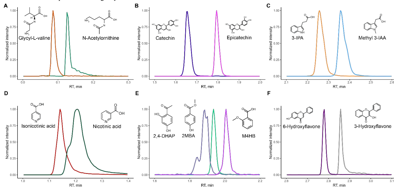
Figure 2 – Separation of 6 sets of isomeric molecules present in the testing library. All data represented is the extracted ion chromatogram acquired in negative mode, with normalized intensity.
