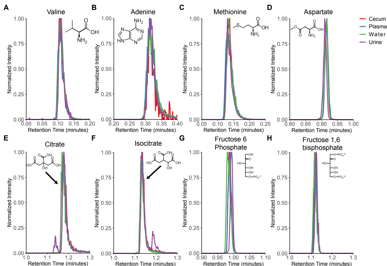
Figure 3 – Extracted ion chromatograms (EICs) in four different matrices.
