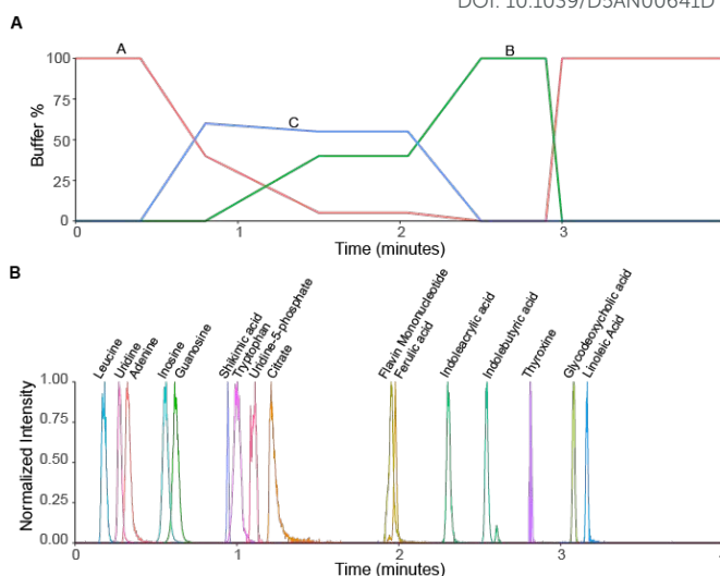
Figure 1 – Representation of mixed-mode chromatographic gradient. (A) Gradient profile with the relative concentrations of solvent A (red): 5 \mu M medronic acid in water, solvent B (green): 0.1% v/v formic acid in methanol; and solvent C (blue): 5 mM ammonium formate and 0.1% v/v formic acid in
