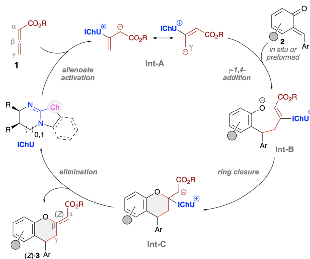
Scheme 5 Mechanistic proposal. 10
