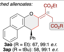
Scheme 4 Asymmetric application scope using in situ generated oQMs (accessed from compounds 7 ) and different allenolates in the presence of (2 S ,3 R )-SeHyperBTM (ISeU; conditions as detailed in entry 9, Table 2).
