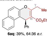
Scheme 4 Asymmetric application scope using in situ generated oQMs (accessed from compounds 7 ) and different allenolates in the presence of (2 S ,3 R )-SeHyperBTM (ISeU; conditions as detailed in entry 9, Table 2).
