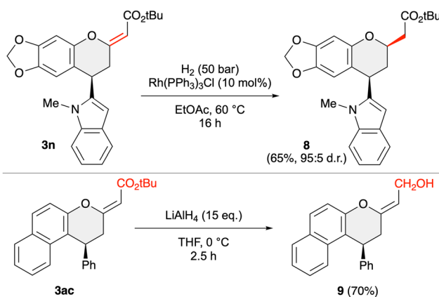
Scheme 6 Reductive follow-up transformations of compounds 3 .
