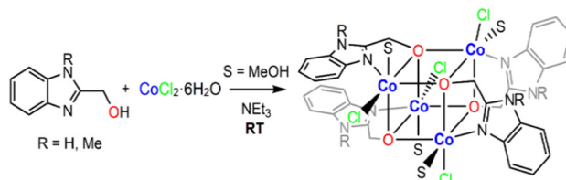
Scheme 1 Self-assembly of [(\mu^3\text{-L}^n\text{O})\text{CoCl}(\text{S})]_4 .
