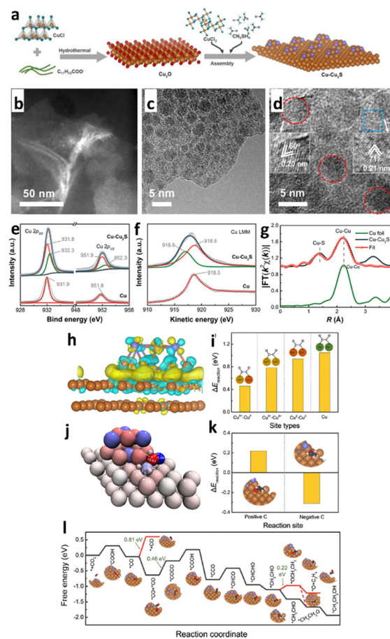
Fig. 18 (a) Schematic illustration of the synthesis of \text{Cu-Cu}_2\text{S} . Characterization of the \text{Cu-Cu}_2\text{S} sample. (b) and (c) TEM, (d) high-resolution TEM (HRTEM), (e) high-resolution Cu 2p XP spectra, (f) Cu LMM Auger spectra, and (g) Cu K-edge K_2 -weighted \chi(k) function of Fourier transform extended X-ray absorption fine structure (EXAFS) spectra of the sample, where pristine Cu and Cu foil are used as controls in panels (e)–(g), revealing that both \text{Cu}(0) and \text{Cu}(I) states are involved, respectively. Calculated \text{ECO}_2\text{R} on \text{Cu-Cu}_2\text{S} . (h) DFT-calculated charge density difference of \text{Cu-Cu}_2\text{S} (the Cu and S atoms are in brown and violet, respectively; the yellow and cyan colours represent charge accumulation and depletion, respectively; the isosurface value is 0.002 \text{ e}^- \text{ \AA}^{-3} ). (i) Energy barrier ( \Delta E_{\text{reaction}} ) for two \text{*CO} forming one \text{*OCCO} via C–C coupling at \text{Cu}^{\delta+}-\text{Cu}^0 , \text{Cu}^{\delta+}-\text{Cu}^{\delta+} , and \text{Cu}^0-\text{Cu}^0 sites of \text{Cu-Cu}_2\text{S} and at the pristine Cu surface, where \text{Cu}^{\delta+} and \text{Cu}^0 of \text{Cu-Cu}_2\text{S} and Cu of pristine are in brown, red, and green, respectively, showing that the energy barrier at the \text{Cu}^{\delta+}-\text{Cu}^0 site of \text{Cu-Cu}_2\text{S} is the lowest. (j) Bader charge of \text{*CH}_2\text{CHO} adsorbed on \text{Cu-Cu}_2\text{S} , where the colour ranging from blue to red indicates the negative to the positive charge of the atoms, respectively. (k) \Delta E_{\text{reaction}} for hydrogenation on the positively charged C and negatively charged C of \text{*CH}_2\text{CHO} converting to \text{CH}_2\text{CH}_2\text{O}^* and \text{CH}_3\text{CHO}^* , respectively. (l) Calculated free energy for each step of the reaction pathway converting \text{CO}_2 to \text{C}_2\text{H}_5\text{OH} on \text{Cu-Cu}_2\text{S} (reproduced with permission from ref. 155, copyright ACS 2023).
