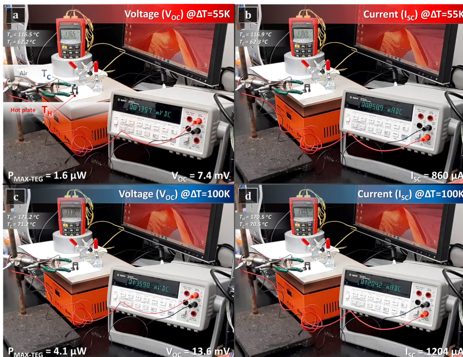
Fig. 8 3D-CTEG-device performance. The generated open-circuit voltage ( V_{\text{OC}} ) and short-circuit current ( I_{\text{SC}} ) at (a, b) \Delta T = 55\text{ K} and (c, d) at \Delta T = 100\text{ K} .
