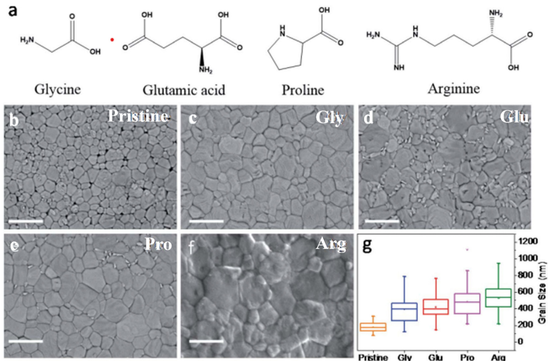
Fig. 6 (a) Chemical structures of the different amino acids and SEM images of (b) pristine and (c) glycine-, (d) glutamic-, (e) proline- and (f) argentine-modified perovskite films; (g) grain sizes of the pristine and modified perovskite films. Reproduced from ref. 99 with permission from Royal Society of Chemistry, Copyright (2021).
