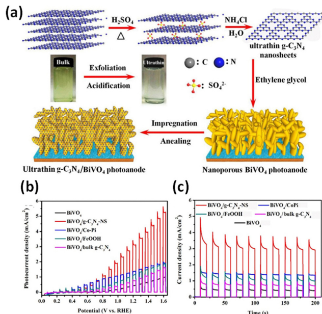
Fig. 7 (a) Schematic illustration of the exfoliation and acidification process for the fabrication of \text{BiVO}_4/g\text{-C}_3\text{N}_4\text{-NS} photoanodes. Reprinted from ref. 240 with permission. (b) J - V curves, (c) transient photocurrent response (1.23 V vs. RHE) for different photoanodes measured under visible-light illumination in 0.1 M \text{Na}_2\text{SO}_4 . Reprinted from ref. 242 with permission.
