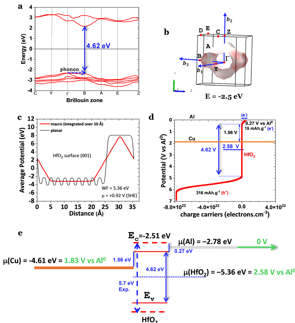
Fig. 3 Electrical and potential energies for \text{HfO}_2 (monoclinic phase P2_1/c ). (a) The electronic band structure (indirect band gap) showing a gap energy of 4.62 \text{ eV} . (b) A surface with E = -2.5 \text{ eV} in the Brillouin zone, approximately the energy of the Fermi surface. (c) The total energy potential of the (001) surface in Fig. 2c where the average potential was integrated over 10 \text{ \AA} , showing a work function, \text{WF} = 5.36 \text{ eV} corresponding to the chemical potential of \mu = +0.92 \text{ V (SHE)} . (d) The chemical potential of \text{HfO}_2 versus \text{Al}^0 , where the \text{Al}^0 chemical potential is E_c(\text{HfO}_2) - \mu(\text{Al}^0) = 0.27 \text{ V} above the minimum energy of the conduction band E_c(\text{HfO}_2) , leading to \text{HfO}_2 likely being reduced by the \text{Al} to a 15 \text{ mAh.g}^{-1} maximum electronic capacity until the chemical potentials of \text{Al} and \text{HfO}_2 equalize. The charge carriers in \text{HfO}_2 are holes, h^+ . From \text{Cu} to \text{HfO}_2 , there are no expected substantial electronic transfers as the valence band of \text{HfO}_2 , as an insulator, is expected to be nearly filled at room temperature, as highlighted by the density of charge carriers being 8 \times 10^{18} \text{ holes cm}^{-3} at OCV, indicating a residual probability of electrons occupying the E_c(\text{HfO}_2) . (e) 1D interpretation of (d), showing absolute chemical potentials for \text{Cu}/\text{HfO}_2/\text{Al} and the conductor and valence bands energies for \text{HfO}_2 for the relative positions of the cell tested by SKP. Note: if the band gap energy of \text{HfO}_2 is 5.7 \text{ eV} , then E_c > \mu(\text{Al}) (dashed line in (d)), and the reduction of \text{HfO}_2 is related to a Schottky barrier of 0.27 \text{ V} = E_c - \mu(\text{Al}) overcome upon charge.
