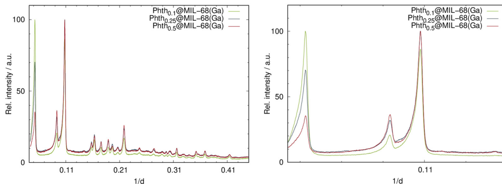
Fig. 5 Left: XRD patterns of the serial dilution of Phth in MIL-68(Ga); right: detailed view of the low angle region of the XRD patterns of Phth x @MIL-68(Ga) (Huber G670: \lambda = 1.54056 \text{ \AA} ; 298 K).
