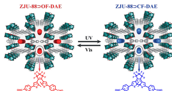
Fig. 22 Structure of LnMOFs and the molecular structures of photoreversible DTEs. Reproduced with permission from ref. 116. Copyright: 2019, Wiley-VCH.
