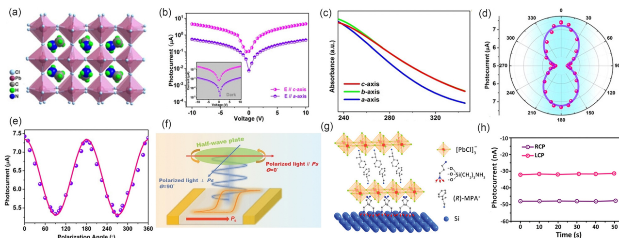
Fig. 4 (a) Structure illumination of (\text{EA})_2(\text{MA})_2\text{Pb}_3\text{Cl}_{10} . (b) I - V curves measured along the c -axis and a -axis under an unpolarized light of 266 nm. (c) Optical absorbance along the three crystallographic axes. (d) Polar plot of the angle-resolved photocurrents. 54 Copyright 2020, Wiley-VCH GmbH. (e) Polarization-dependent photocurrents. (f) Schematic illustration of the polarized-light device of (\text{isobutylammonium})_2(\text{methylammonium})\text{Pb}_2\text{Cl}_7 . 58 Copyright 2022, Wiley-VCH GmbH. (g) Structural illustration of the [(\text{R})\text{-MPA}]_2\text{PbCl}_4/\text{Si} heterostructure. (h) Photocurrent of the device under RCP and LCP illumination. 60 Copyright 2021, Wiley-VCH GmbH.
