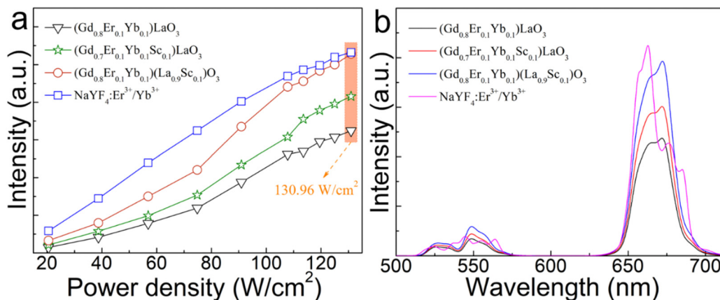
Fig. 5 (a) Red UCL integral intensity of (Gd 0.8 Er 0.1 Yb 0.1 )LaO 3 , (Gd 0.7 Er 0.1 Yb 0.1 Sc 0.1 )LaO 3 , (Gd 0.8 Er 0.1 Yb 0.1 )(La 0.9 Sc 0.1 )O 3 , and commercial β-NaYF 4 :Er 3+ /Yb 3+ phosphors under 980 nm laser excitation with different excitation power densities. (b) UCL spectra when the pump power density of the 980 nm laser was fixed at 130.96 W cm -2 .
