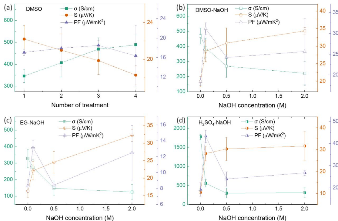
Fig. 7 The variation in electrical conductivity, Seebeck coefficient, and power factor of PEDOT:PSS/40 wt% BST thin films post-treated with: (a) 40 vol% DMSO (1 to 4 rounds), (b) 40 vol% DMSO (3 rounds) and various concentrations of NaOH (1 round), (c) 40 vol% EG (3 rounds) and various concentrations of NaOH (1 round), and (d) 0.5 M \text{H}_2\text{SO}_4 (3 rounds) and various concentrations of NaOH (1 round) at room temperature. The error bars on experimental data were calculated based on three repetitions of measurements on the samples.
