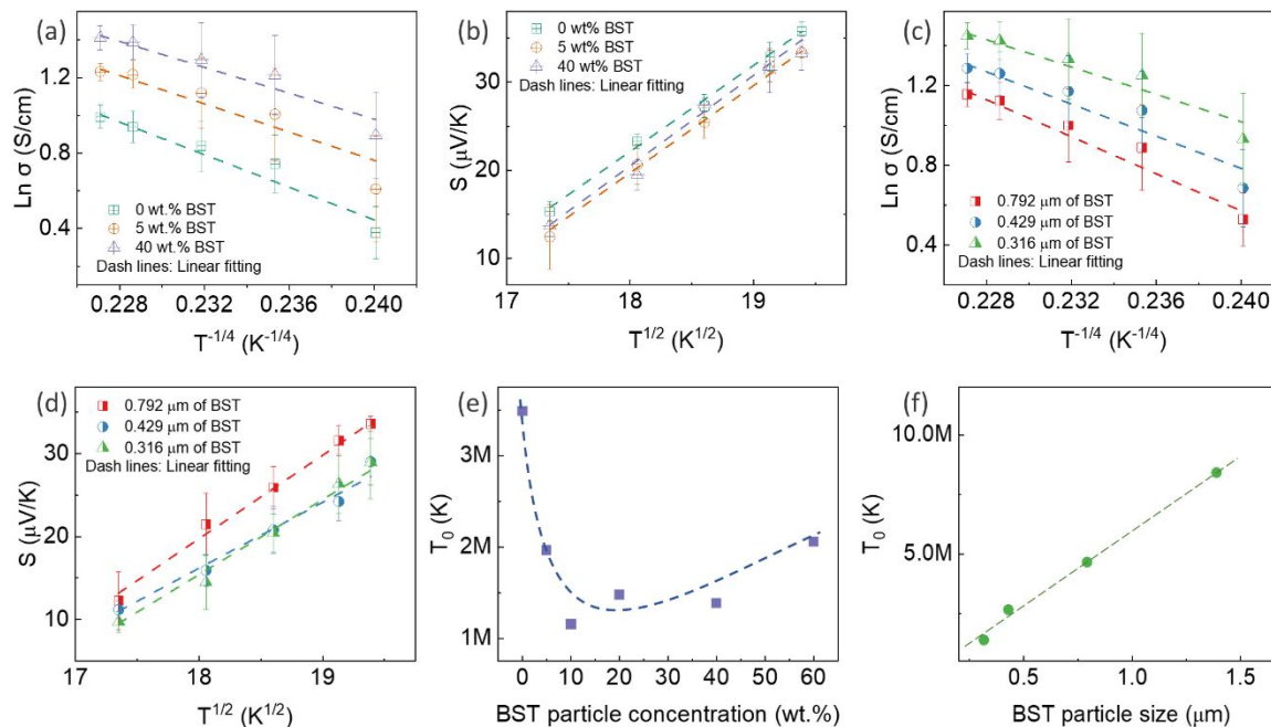
Fig. 4 \ln \sigma as a function of T^{-1/4} , and S as a function of T^{1/2} for PEDOT:PSS/BST thin films with various (a, b) BST concentrations, (c, d) BST particle sizes (The dashed lines in (a-d) represent linear fits to the Mott VRH model of the experimental data). The derived T_0 for PEDOT:PSS/BST thin films with various (e) BST concentrations, (f) BST particle sizes (The dashed lines in (e, f) indicate the eye-tracking). The error bars on experimental data were calculated based on three measurement repetitions on two sets of samples in each case.
