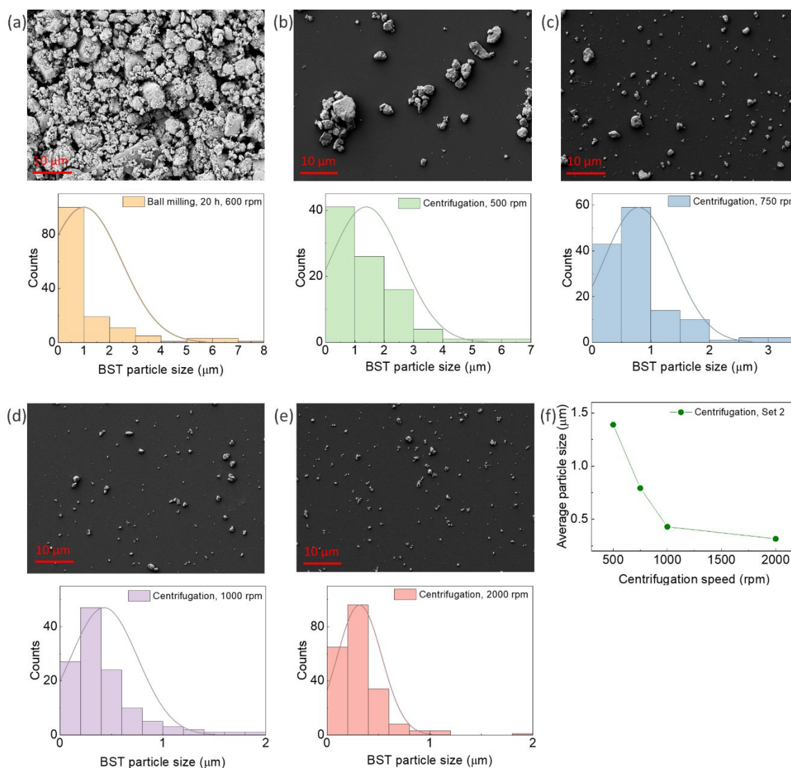
Fig. 1 SEM micrograph and particle size distribution of BST powder produced by (a) ball milling for 20h, 600 rpm, and Set2 centrifugation at four speeds sequentially: (b) 500 rpm, (c) 750 rpm, (d) 1000 rpm, and (e) 2000 rpm. (f) The variation of average particle size with centrifugation speed.
