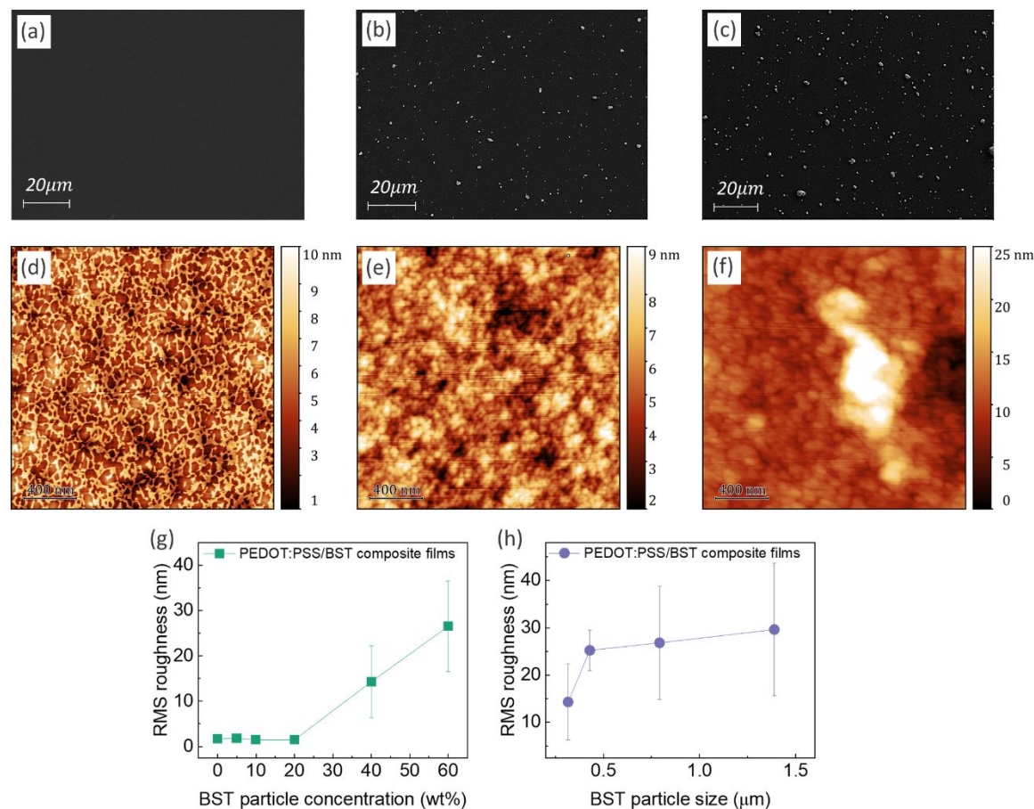
Fig. 2 (a-c) SEM micrographs of PEDOT:PSS thin films with 0, 20, and 40 wt% BST, respectively. (d-f) Corresponding AFM images of the films. The RMS roughness of the films vs (g) BST concentration, and (h) average size of BST particles. All the scan areas are: 2 \times 2 \mu\text{m}^2 . The error bars in (g) and (h) were calculated using RMS values obtained from two different AFM images, with scan areas of 2 \times 2 \mu\text{m}^2 and 5 \times 5 \mu\text{m}^2 .
