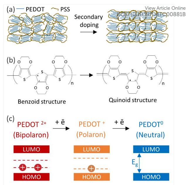
Fig. 6 (a) Schematic diagram illustrating morphological changes in PEDOT:PSS films by secondary doping. (b) Conformational changes in PEDOT from benzoid to quinoid structure. (c) Transition of PEDOT chains from bipolaron to polaron and neutral states during the dedoping process.
