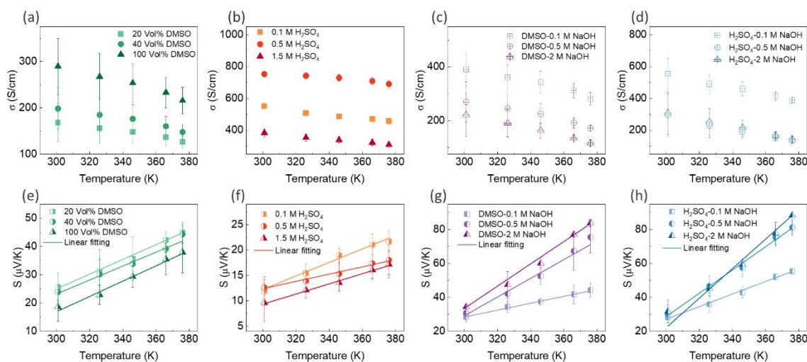
Fig. 8 The variation of electrical conductivity and Seebeck coefficient with temperature for PEDOT:PSS/40 wt% BST thin films after: single post-treatment with DMSO (a, e), \text{H}_2\text{SO}_4 (b, f), sequential post-treatment with DMSO-NaOH (c, g), and \text{H}_2\text{SO}_4 -NaOH (d, h). The dash lines in (e-h) represent the linear fitting of equation (7) to the experimental data. The error bars on experimental data were calculated based on three repetitions of measurements on the samples.
