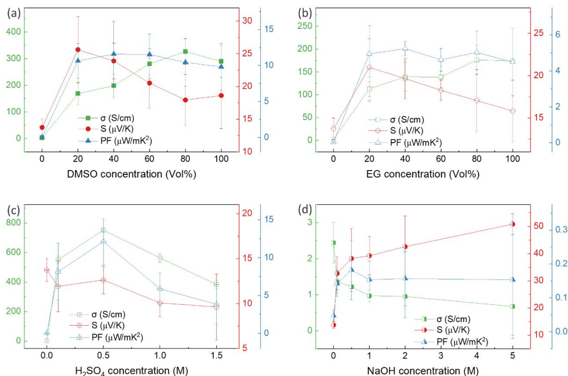
Fig. 5 The variation in electrical conductivity, Seebeck coefficient, and power factor of single post-treated PEDOT:PSS thin films with: (a) DMSO, (b) EG, (c) \text{H}_2\text{SO}_4 , and (d) NaOH concentrations at room temperature. The error bars on experimental data were calculated based on three repetitions of measurements on the samples.
