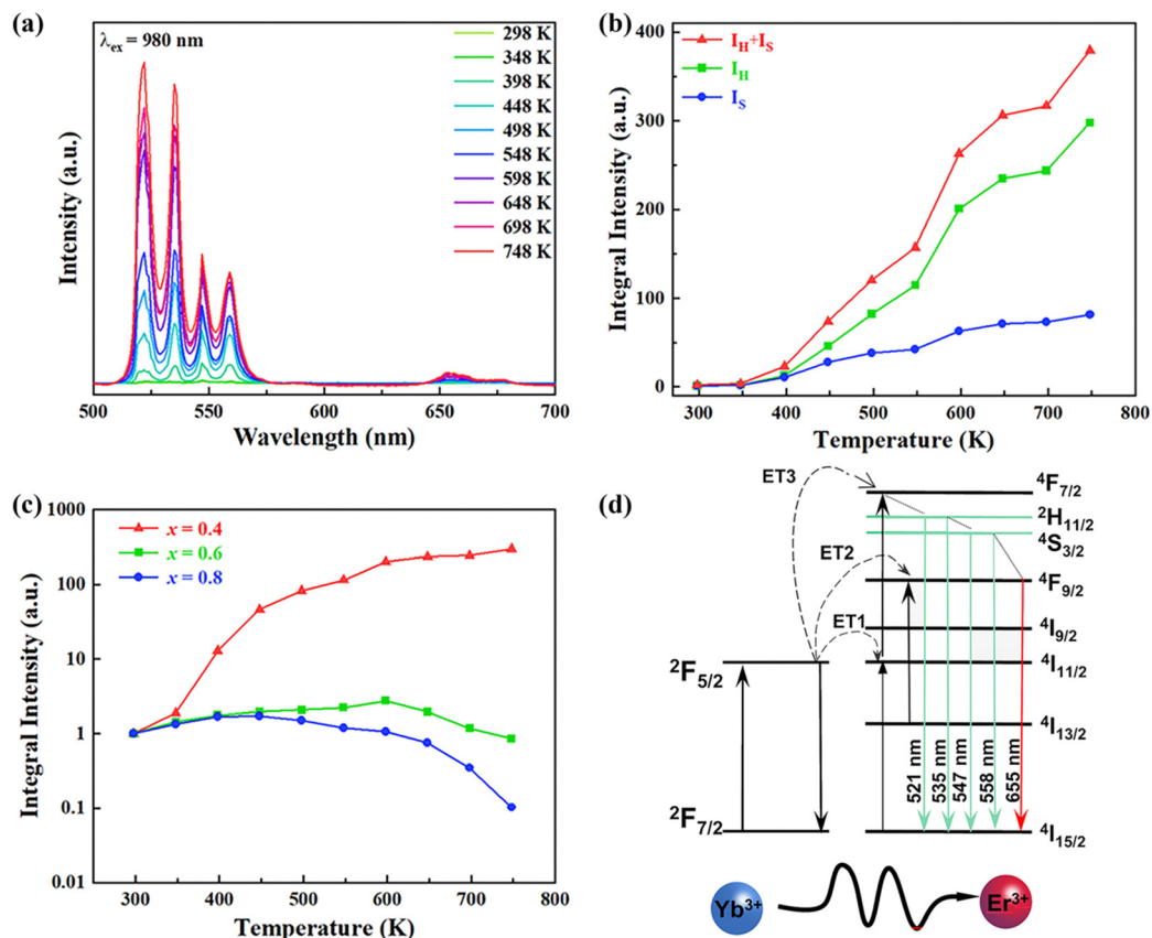
Fig. 6 (a) UCL emission spectra of the KM4 sample at 298–748 K under 980 nm laser excitation. (b) The corresponding UCL emission integral intensities of ^2\text{H}_{11/2}/^2\text{H}_{11/2(1)} , ^4\text{S}_{3/2}/^4\text{S}_{3/2(1)} and total ( ^2\text{H}_{11/2} + ^4\text{S}_{3/2} ) levels of \text{Er}^{3+} ions. (c) Integral intensity of KM4, KM6, and KM8 samples as a function of temperature. (d) Simplified energy level diagram to describe the ET process in the KM4 sample.
