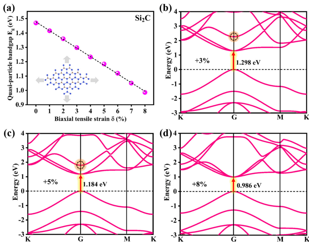
Fig. 4 (a) Quasi-particle energy bandgap as a function of tensile strain \delta for the Si 2 C monolayer. (b)–(d) Quasi-particle band structures of the Si 2 C monolayer at tensile strains of +3%, +5%, and +8%.
