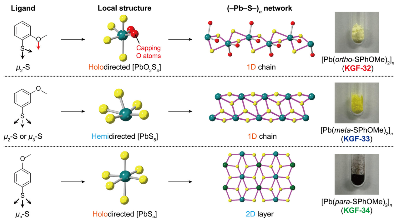
Fig. 1 Schematic illustration of structures for [\text{Pb}(x\text{-SPhOMe})_2]_n ( x = \text{ortho} ( KGF-32 ), \text{meta} ( KGF-33 ), and \text{para} ( KGF-34 )). From left to right: Coordination modes of SPhOMe ligands, local structures around Pb(II) ions, (-\text{Pb}-\text{S})_n dimensionality, photographs of corresponding samples.
