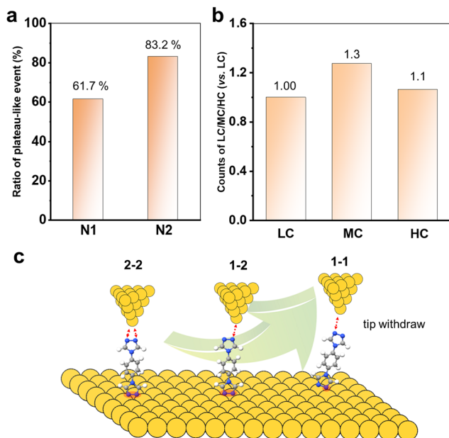
Fig. 4 (a) The percentage of plateau-like events in the conductance traces for N1 and N2 . (b) Relative count ratios of LC, MC and HC plateau-like events for N2 . (c) Schematic of the molecular junction formation mechanism during withdrawing the tip from the substrates with adsorption of N2 .
