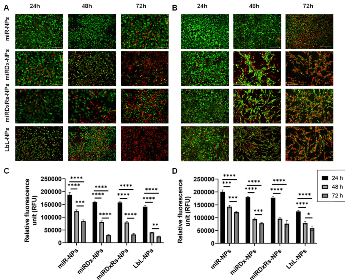
Fig. 5 Live/dead images of U2OS (A) and Saos-2 cells (B) incubated with all the manufactured NPs for 24, 48 and 72 h. Bar = 300 μm; metabolic activity of U2OS (C) and Saos-2 (D) cells incubated with all the manufactured NPs for 24, 48 and 72 h. The results are shown as average ± SD.
