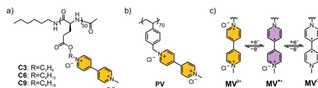
Fig. 2 The chemical structure of (a) viologen-based polypeptides with alkyl spacer lengths of three (C3), six (C6), or nine (C9) carbons. (b) The chemical structure of the control viologen (PV), bearing a non-peptide backbone. (c) The redox reaction of methyl viologen consisting of the dication ( \text{MV}^{2+} ), radical cation ( \text{MV}^{+\cdot} ), and the neutral ( \text{MV}^0 ) states.
