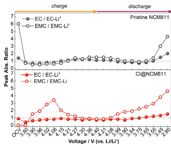
Fig. 6 \text{Li}^+ solvation behavior comparison of (a) pristine NCM811 and (b) CI@NCM811 represented by a ratio of \text{EC}/\text{EC-Li}^+ and \text{EMC}/\text{EMC-Li}^+ . EC is present at 1806\text{ cm}^{-1} , \text{EC-Li}^+ at 1773\text{ cm}^{-1} , EMC at 1747\text{ cm}^{-1} , and \text{EMC-Li}^+ at 1717\text{ cm}^{-1} .
