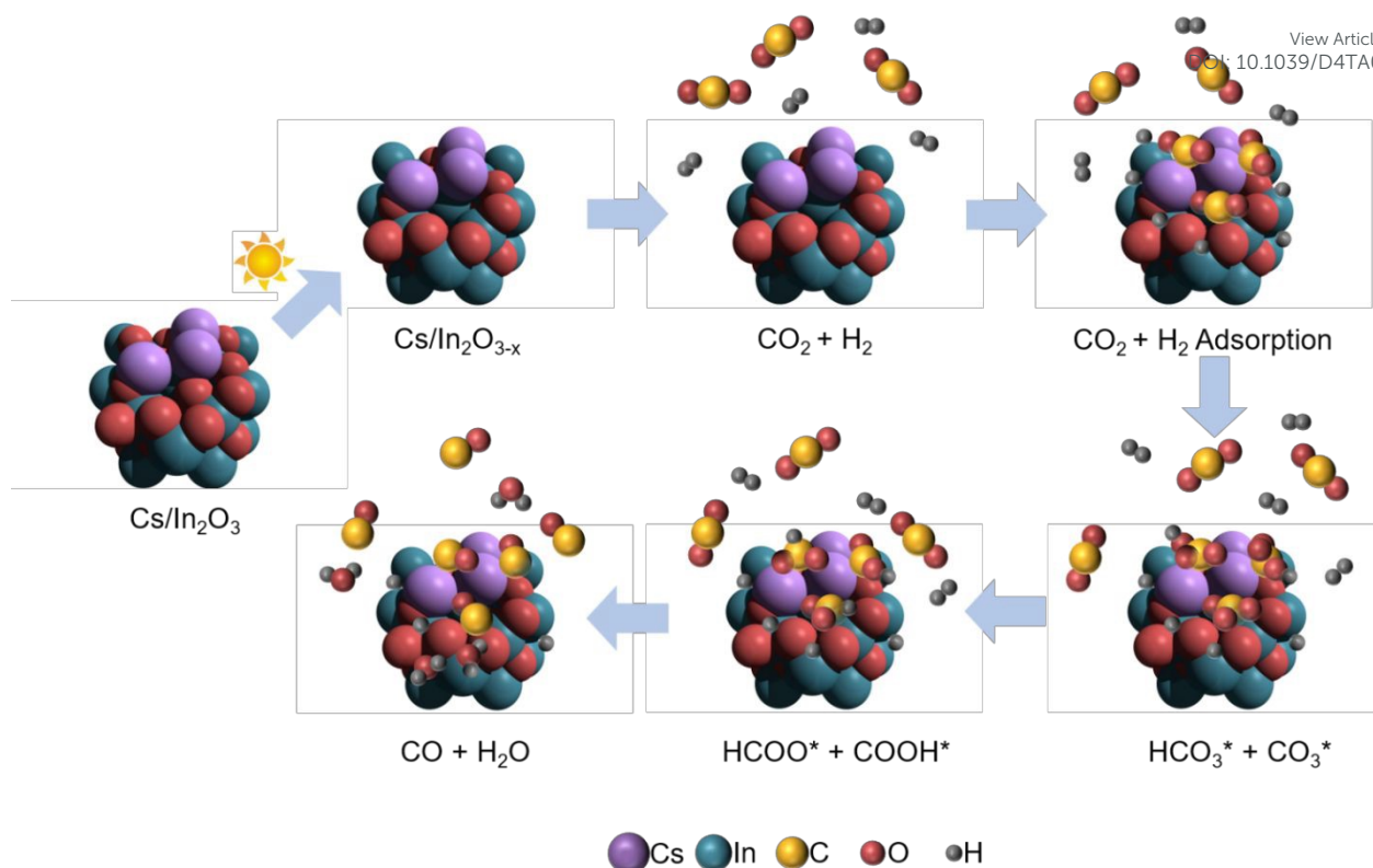
Fig. 5 Schematic illustration for the proposed reaction mechanism of the photo-thermal \text{CO}_2 hydrogenation over Cs-promoted \text{In}_2\text{O}_3 .
