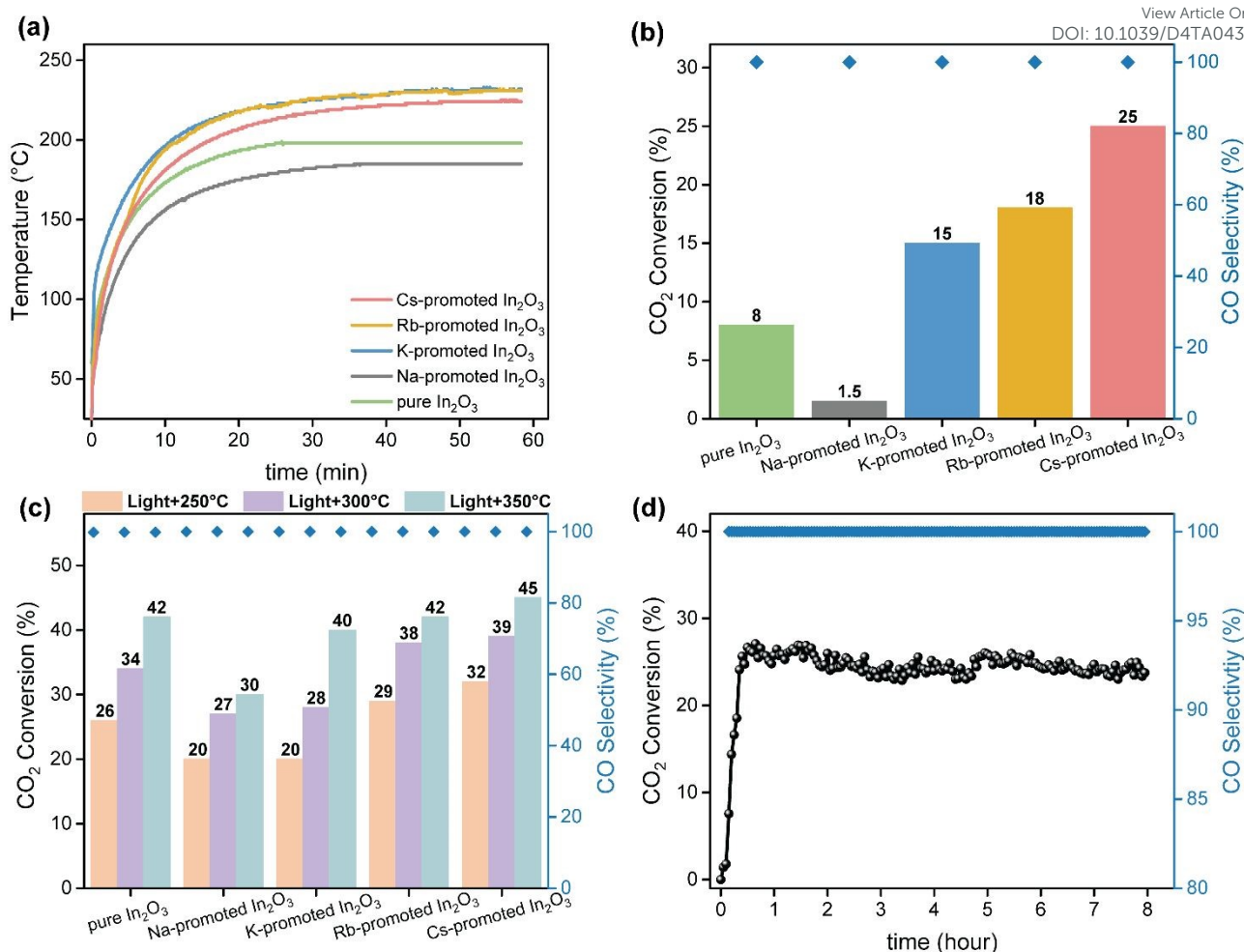
Fig. 2 a) Temperature evolution over pure and alkali-promoted catalysts under 3.3 \text{ W}\cdot\text{cm}^{-2} light irradiation. b) CO 2 conversion and CO selectivity over pure and alkali-promoted \text{In}_2\text{O}_3 without external heating under irradiation of 3.3 \text{ W}\cdot\text{cm}^{-2} . Reaction conditions: GSHV = 15000 \text{ mL}\cdot\text{h}^{-1}\cdot\text{g}^{-1} , 1 bar. c) CO 2 conversion and CO selectivity over pure and alkali promoted \text{In}_2\text{O}_3 with external heating at 250, 300 and 350 °C under irradiation of 3.3 \text{ W}\cdot\text{cm}^{-2} . Reaction conditions: GSHV = 15000 \text{ mL}\cdot\text{h}^{-1}\cdot\text{g}^{-1} , 1 bar. d) Stability test of Cs-promoted \text{In}_2\text{O}_3 with external heating at 250 °C under irradiation of 3 \text{ W}\cdot\text{cm}^{-2} . Reaction conditions: GSHV = 15000 \text{ mL}\cdot\text{h}^{-1}\cdot\text{g}^{-1} , 1 bar.
