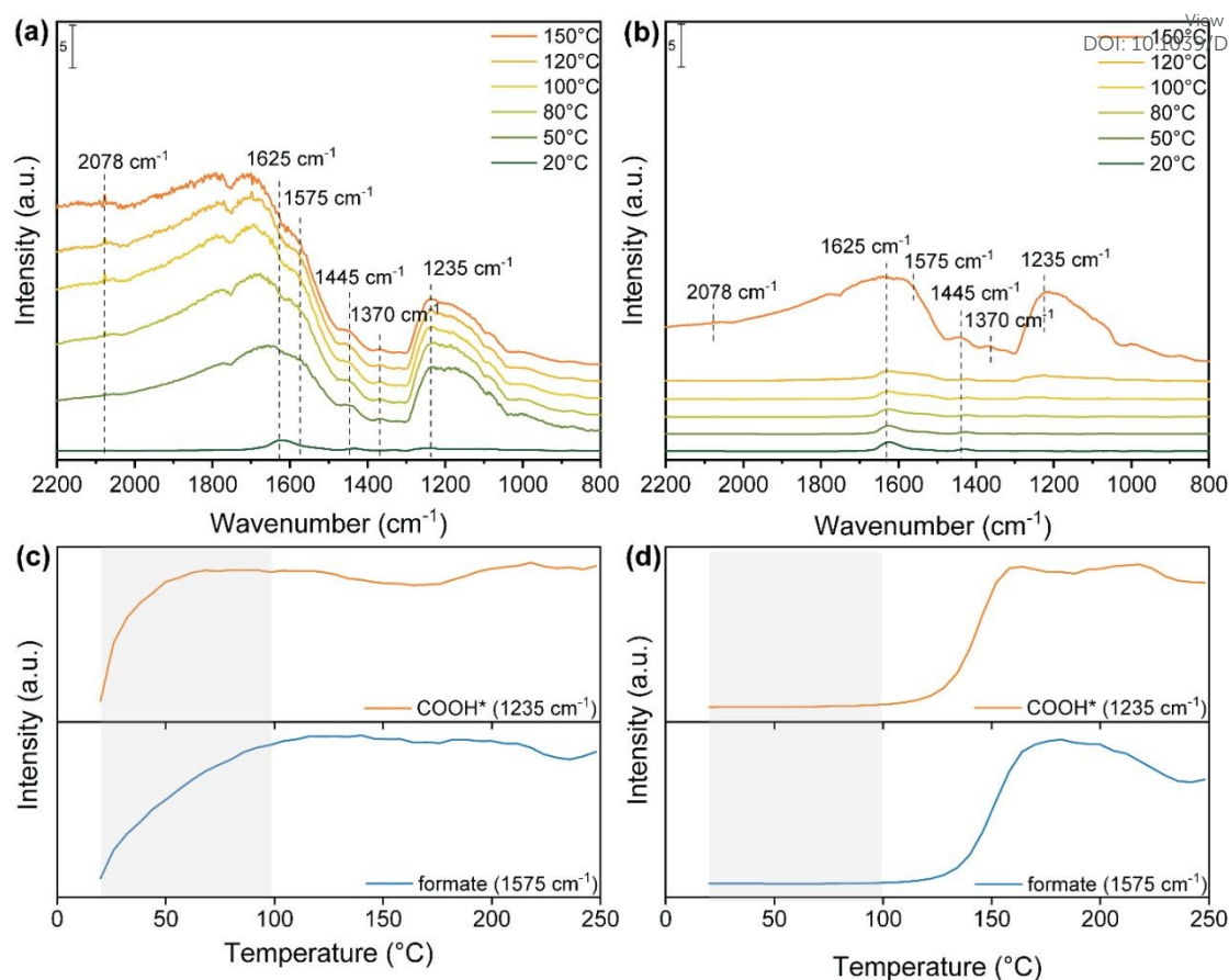
Fig. 4 In-situ DRIFTS spectra of Cs-promoted \text{In}_2\text{O}_3 under \text{H}_2 and \text{CO}_2 (4:1) at 10 bar with increased temperature upon a) light and b) dark conditions. IR peak intensities of \text{COOH}^* and bidentate formate species as a function of temperature under c) light and d) dark conditions.
