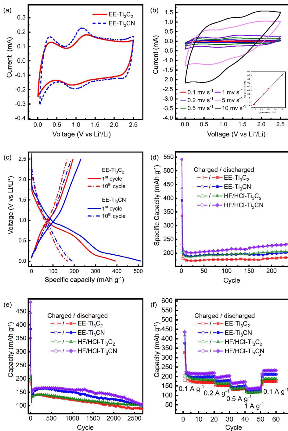
Fig. 4 (a) CV curves of EE-Ti 3 C 2 and EE-Ti 3 CN from 2.5 V to 0.05 V vs. Li + /Li + , obtained at a scan rate of 0.5 mV s -1 . (b) CV curves of EE-Ti 3 C 2 at various scan rates. (c) Galvanostatic charge–discharge profiles of EE-Ti 3 C 2 and EE-Ti 3 CN at a current density of 0.1 A g -1 . (d) Cycle performance of EE-Ti 3 C 2 , EE-Ti 3 CN, HF/HCl-Ti 3 C 2 , and HF/HCl-Ti 3 CN at a current density of 0.1 and (e) 1 A g -1 . (f) Rate capability test of EE-Ti 3 C 2 and EE-Ti 3 CN and their HF/HCl etched analogs at 0.1, 0.2, 0.5, and 1 A g -1 .
