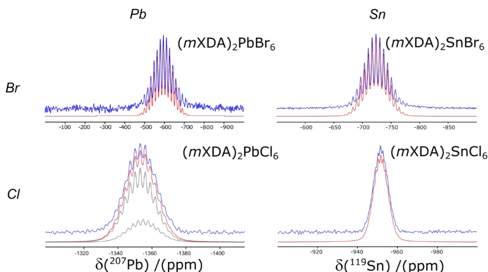
Figure 5. The ^{207}\text{Pb} MAS NMR spectra of (\text{mXDA})_2\text{PbBr}_6 and (\text{mXDA})_2\text{PbCl}_6 and the ^{119}\text{Sn} CPMAS NMR spectra of (\text{mXDA})_2\text{SnBr}_6 and (\text{mXDA})_2\text{SnCl}_6 . Experimental spectra, simulated spectra and deconvoluted resonances are displayed in blue, red and grey respectively.
