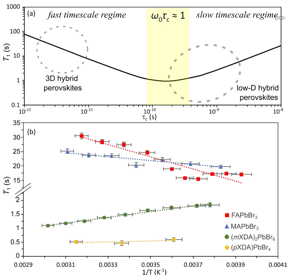
Figure 4. (a) Schematic of the ideal ^1\text{H} T_1 -correlation time relationship for dipolar mediated relaxation following Equation 2 at 14.1 T, using a representative inter-moment distance r = 2 Å, to demonstrate the different timescale regimes. (b) Plot of ^1\text{H} T_1 versus inverse temperature for FAPbBr 3 , MAPbBr 3 , (mXDA) 2 PbBr 6 , and (pXDA)PbBr 4 .
