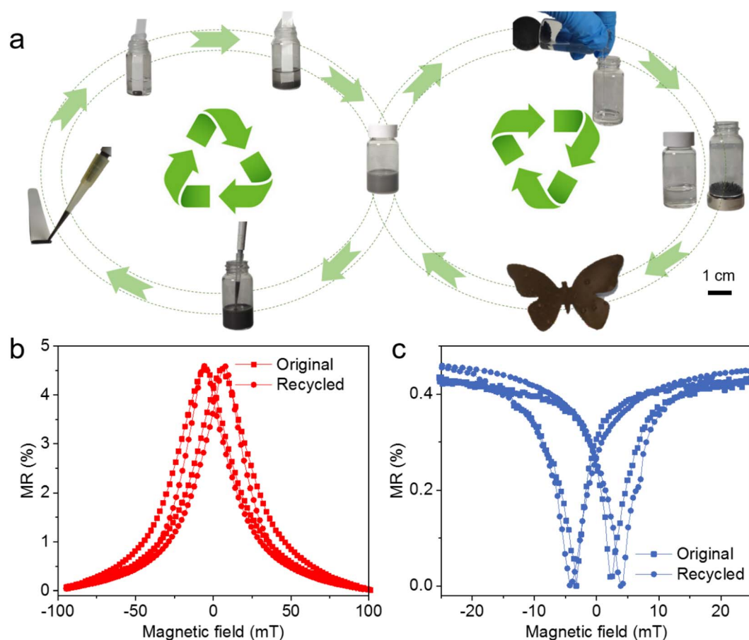
Fig. 4 Recyclable properties of printed magneto-resistive sensors. (a) The left loop illustrates the recycling and reproduction process of printed magneto-resistive sensors: discarded sensors are immersed in solvent to decompose magneto-resistive fillers and polymer binders, after which the recycled ink is used to fabricate new sensors. The right loop illustrates the separation of component materials and the fabrication of a magnetic soft robot using the separated polymers and magnetic fillers. (b and c) MR response of the printed sensors with the recycled materials. The sensors exploit (b) GMR microflakes and (c) AMR microparticles as fillers.
