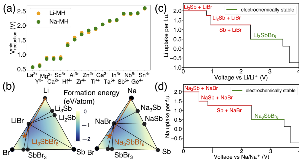
Fig. 5 (a) The minimum reduction potential of Li metal halide and Na metal halide compounds and (b) phase diagram of Li–Sb–Br and Na–Sb–Br. The formation energy of compositions in the phase diagram is illustrated by a color gradient, and its value is marked by the color contour. The stable phases are shown by black circles, the target compounds are marked as orange stars and the orange arrows illustrate the decomposition pathways of \text{Li}_3\text{SbBr}_8 and \text{Na}_3\text{SbBr}_8 . The equilibrium voltage profiles and phase equilibria for lithiation reactions of (c) \text{Li}_3\text{SbBr}_8 and (d) \text{Na}_3\text{SbBr}_8 , respectively. The decomposition products of lithiation reactions at the anode side are labeled in red color, and the electrochemically stable voltage range is marked in green color.
