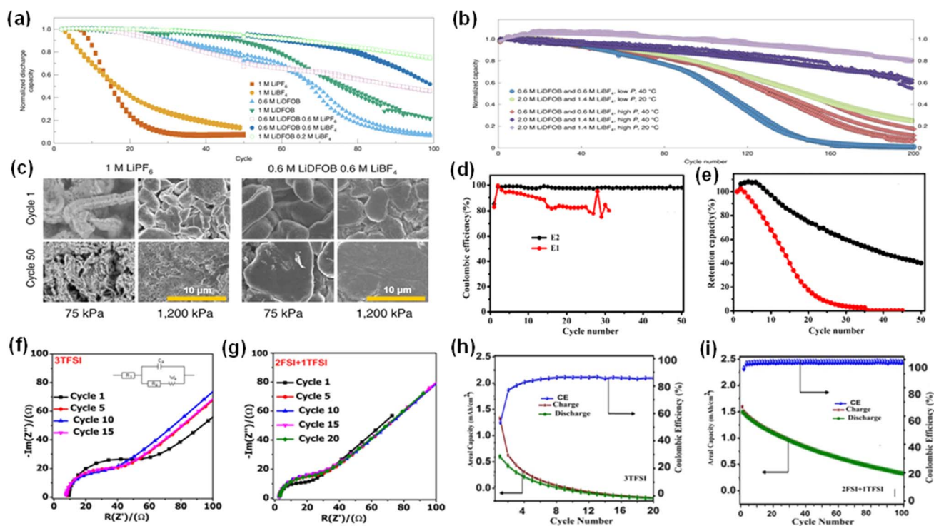
Fig. 3 Electrochemical performance of batteries with newly developed liquid electrolytes. (a) Cycling stability of cells with different ratios of electrolytes. (b) Capacity retentions of cells using different concentrations of LiDFOB and \text{LiBF}_4 at various pressures and temperatures. 24 Reproduced with permission. Copyright 2020, Springer Nature. (c) SEM images of the Li layer in AFLMBs employing two different electrolytes and cycling pressures. 21 Reproduced with permission. Copyright 2019, Springer Nature. (d and e) Comparing CE and capacity retention of \text{Cu}||\text{NMC} cells employing 1 M \text{LiPF}_6 in EC/DEC (E1) and 2 M \text{LiPF}_6 in EC/DEC (E2). 30 Reproduced with permission. Copyright 2019, the American Chemical Society. (f and g) Electrochemical impedance spectroscopy comparison of AFLMBs with a 3 M LiTFSI and a dual-salt of 2 M LiFSI + 1 M LiTFSI. (h and i) Cycling performances of anode-free cells with the single salt and the dual-salt. 33 Reproduced with permission. Copyright 2019, Electrochemical Society, Inc.
