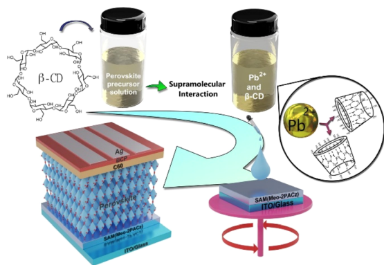
Scheme 1 Representation of \beta -CD modulation mechanism and potential interaction sites in an inverted perovskite solar cell.
