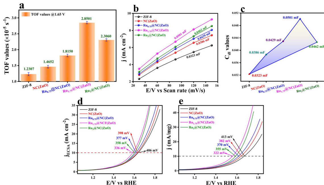
Fig. 4 (a) TOF values of ZIF-8, NC(ZnO), Ru 0.75 @NC(ZnO), Ru 1.75 @NC(ZnO) and Ru 3 @NC(ZnO); (b) C_{dl} values measured from the CV curves; (c) comparison of the C_{dl} values; (d) ECSA normalized (specific activity) LSV polarization results; (e) mass dependent activity of all the catalysts.
