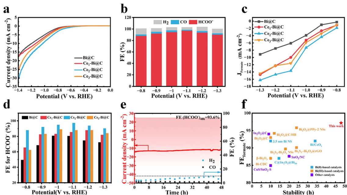
Fig. 3 Electrochemical measurements. (a) LSV curves of Bi@C, Ce 1 -Bi@C, Ce 2 -Bi@C and Ce 3 -Bi@C in CO 2 -saturated 0.1 M KHCO 3 . (b) Faradaic efficiencies of the reduction products generated by Ce 2 -Bi@C in 0.1 M CO 2 -saturated KHCO 3 aqueous solution at different applied potentials. (c) HCOO - partial current densities and (d) potential-dependent FEs of HCOO - for Bi@C, Ce 1 -Bi@C, Ce 2 -Bi@C and Ce 3 -Bi@C. (e) Amperometric i - t stability of Ce 2 -Bi@C in 0.1 M KHCO 3 at -1.1 V vs. RHE. (f) Comparison of FE formate and stability for Ce 2 -Bi@C and some recently reported catalysts for the CO 2 RR.
