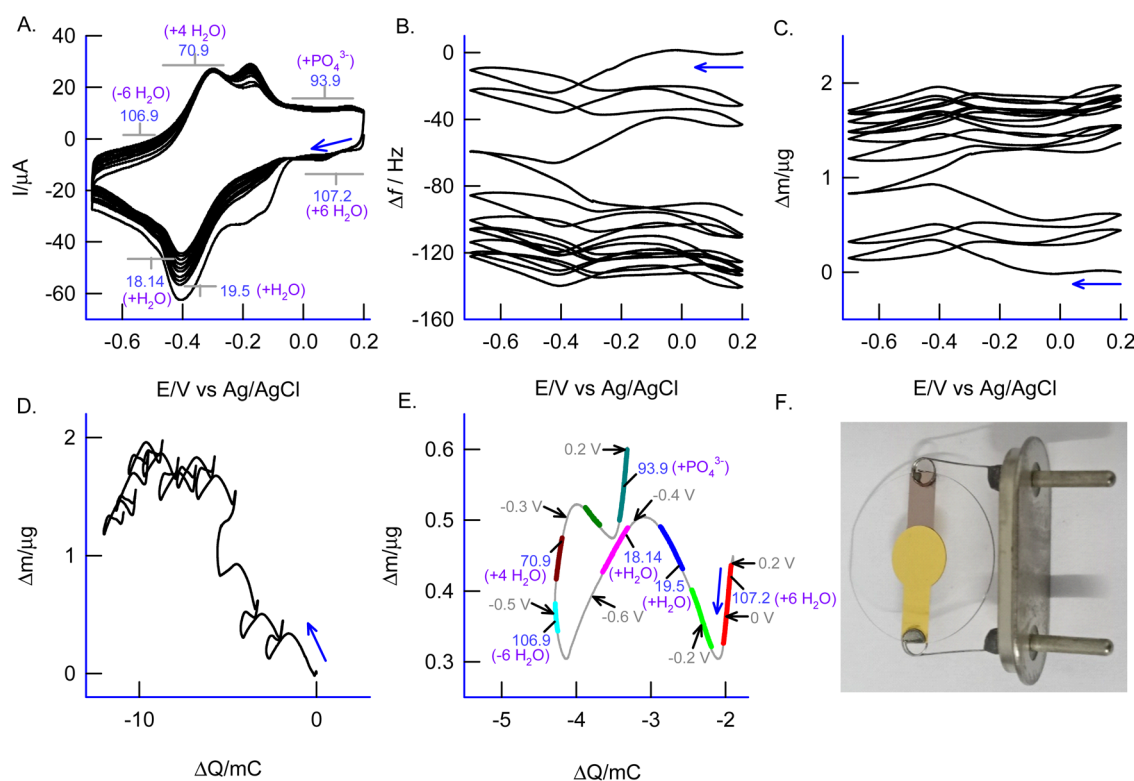
Fig. 5 (A and B) In situ CV-EQCM responses of \text{GCE/GMC}@\{\text{Cu}(\text{BPA})\text{Cl}\}_{\text{ads}} in \text{N}_2 purged 0.1 M PBS, pH 7, at a scan rate of 10\text{ mV s}^{-1} . Inset of (A) shows the molecules involved in the redox reaction. Corresponding derivative plots of (C) \Delta m vs. E and \Delta m vs. \Delta Q plots of (D) 1–10 cycles and (E) second cycle. (F) Picture of an EQCM-Au electrode.
