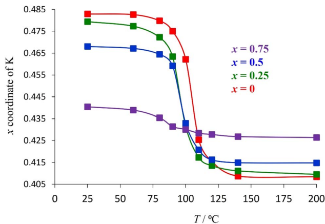
Fig. 9 The temperature dependence of the potassium coordinate ( x, x, x ) in as-prepared K_{1-x}Cs_xTa_{0.5}Nb_{0.5}WO_6 ( 0 \leq x \leq 0.75 ), determined from Rietveld analysis of synchrotron powder X-ray diffraction data collected at temperatures in the range 25 \leq T/^\circ C \leq 200 . The error bars lie within the points.
