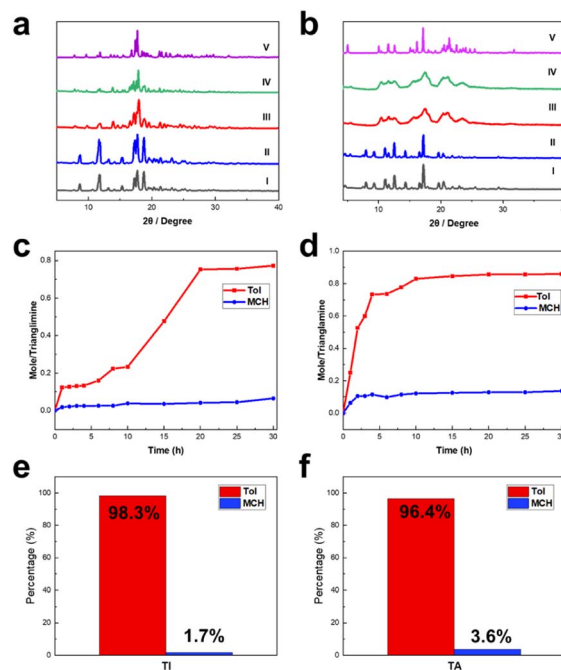
Fig. 4 (a) PXRD pattern of TI: (I) pure activated TI, (II) after absorption of MCH, (III) after absorption of Tol, (IV) after absorption of the Tol/MCH mixture, and (V) simulated from the single crystal structure of Tol@TI. (b) PXRD pattern of TA: (I) pure activated TA, (II) after absorption of MCH, (III) after absorption of Tol, (IV) after absorption of the Tol/MCH mixture, and (V) simulated from the single crystal structure of Tol@TA. (c) Time-dependent solid-vapor sorption curve of TI with a mix component of Tol/MCH. (d) Time-dependent solid-vapor sorption curve of TA with a mix component of Tol/MCH. (e) Relative uptakes of Tol/MCH in TI after saturated absorption. (f) Relative uptakes of Tol/MCH in TA after saturated absorption.
