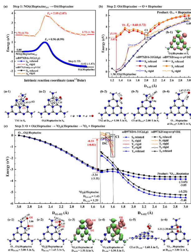
Fig. 3 The DFT-calculated energy profiles of (a) step 1: N of NO intercalation into heptazine NV in S 0 and S 1 states with the (a-1) TS1 and (a-2) O@heptazine in S 0 ; (b) step 2: O-desorption from heptazine in S 0 and S 1 , with the (b-1) spatial distribution of the photo-induced hole (pink) and electron (green) (isovalue = 0.002 a.u.) of O@heptazine in S 1 , (b-2) TS2 at the N-O distance of NO ( D_{N-O} ) = 1.50 Å in S 1 , (b-3) approximate Cl-point at D_{N-O} = 2.00 Å in S 1 , and (b-4) O··heptazine at D_{N-O} = 3.00 Å in S 0 ; and (c) step 3: the combination of the hydrogen-bonding O with O@heptazine to release triplet 3 O 2 under illumination, with the (c-1) O··O@heptazine at D_{O1-O2} = 3.00 Å in S 0 , (c-2) 1 O 2 @heptazine at D_{O1-O2} = 1.43 Å in S 0 , spatial distribution of the photo-induced hole (pink) and electron (green) (isovalue = 0.002 a.u.) at D_{N-O2} = 1.50 Å in (c-3) S 1 and (c-4) T 1 , (c-5) approximate Cl-point at D_{N-O2} = 1.60 Å in T 0 , and (c-6) 3 O 2 ··heptazine at D_{N-O2} = 3.00 Å in T 0 . The filled symbols refer to the relaxed scanning ( i.e. constrained optimizations) by manually fixing the D_{N-O} as 1.20–3.00 Å, D_{O1-O2} as 3.00–1.43 Å, or D_{N-O2} as 1.38–3.00 Å, while hollow symbols refer to the rigid scanning ( i.e. single-point energy calculations) based on the optimized geometries. The key energies E (unit: eV) and interatomic distances (unit: Å) are marked. The data obtained by ωB97XD/aug-cc-pVDZ are labeled in brackets only if the results differ from those by ωB97XD/6-31G(d,p).
